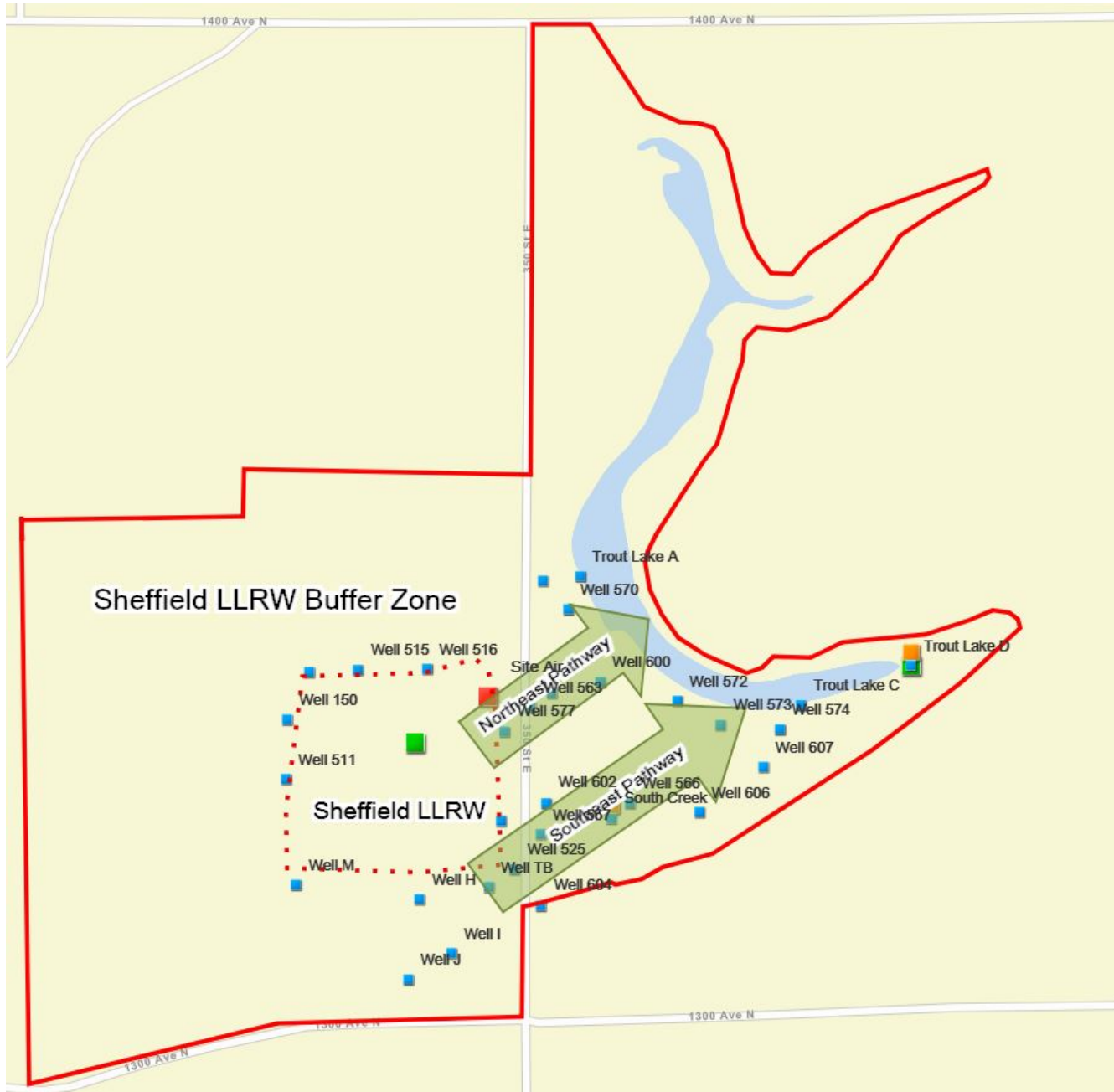
Figure A-1. Sheffield Site and Approximate Groundwater Pathways
